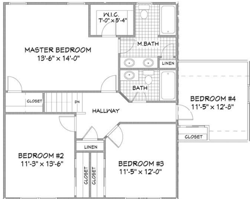
SECOND FLOOR (1,057 SQ.FT.)
