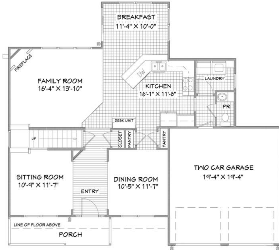
FIRST FLOOR (1,090 SQ.FT.)
