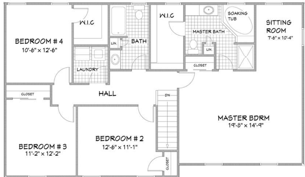
SECOND FLOOR (1,298 SQ.FT.)
