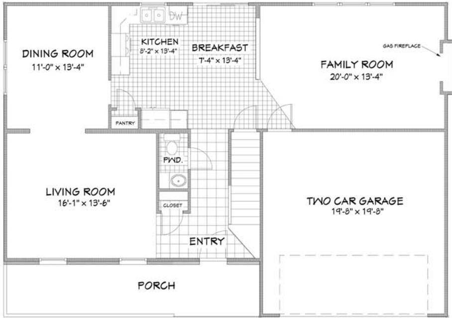
FIRST FLOOR (1,054 SQ.FT.)
