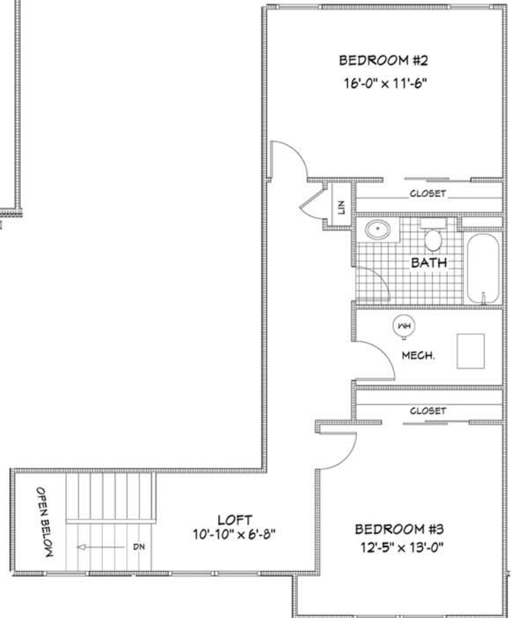
SECOND FLOOR (769 SQ.FT.)
