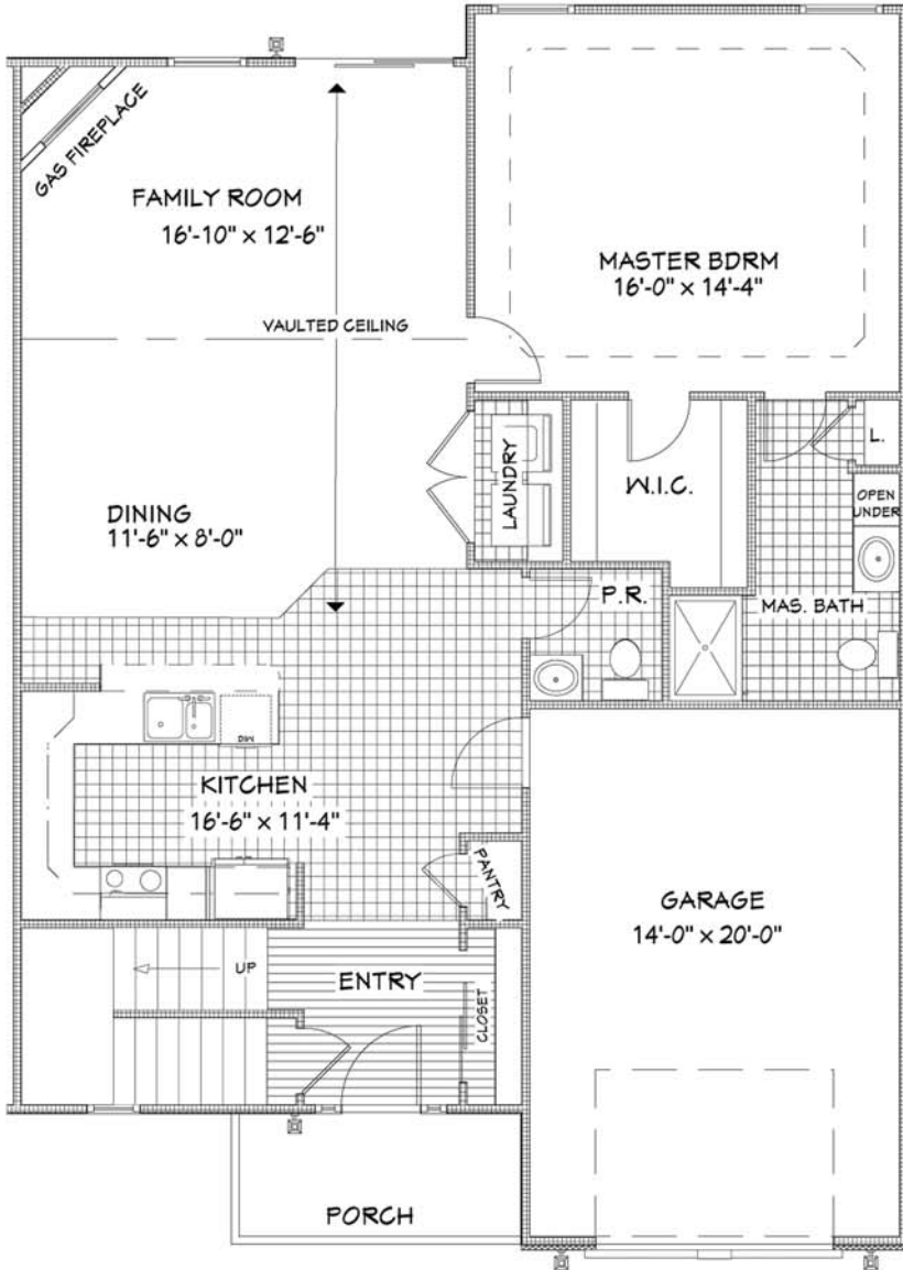
FIRST FLOOR (1,166 SQ.FT.)
