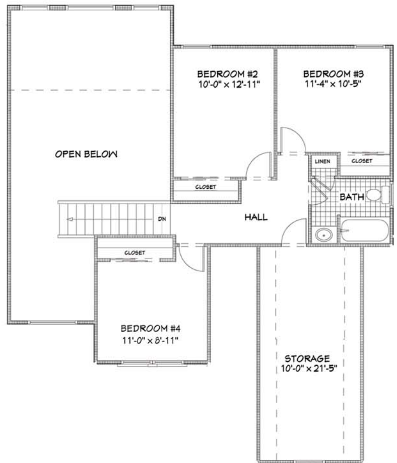
SECOND FLOOR (623 SQ.FT.)
