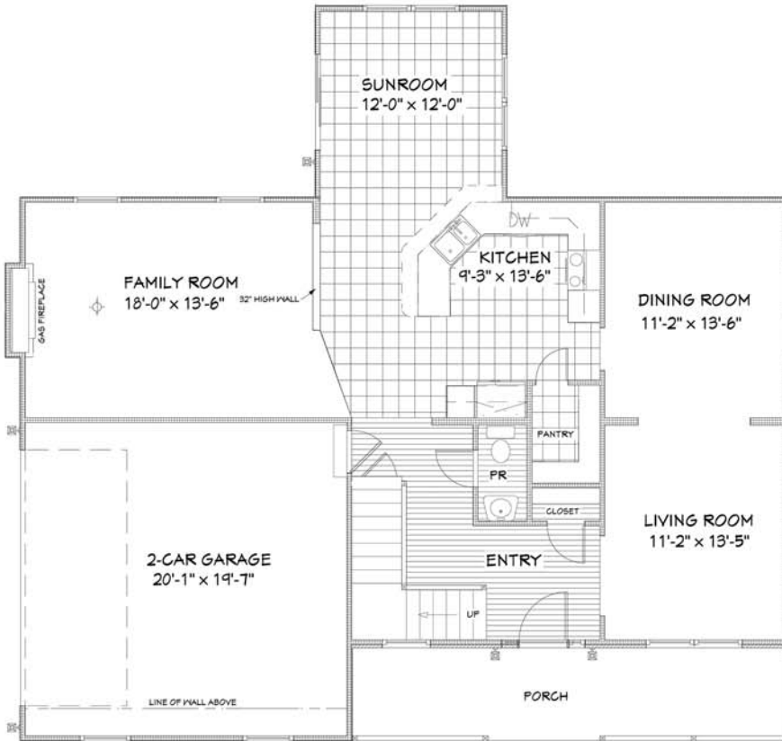
FIRST FLOOR (1,197 SQ.FT.)
